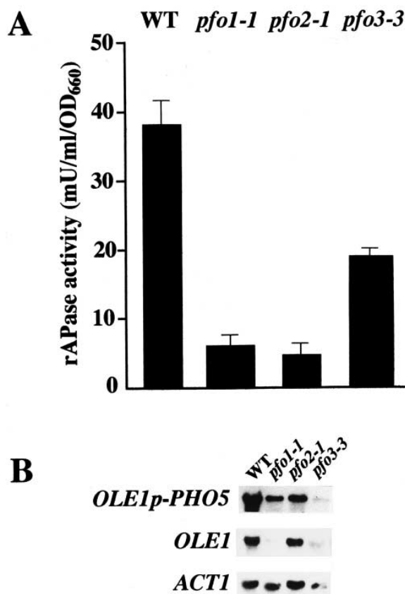
Fig. 2. rAPase activity and Northern analysis of the OLE1 and OLE1p-PHO5 transcripts of the wild-type and pfo mutants. A : rAPase activity from the OLE1p-PHO5 fusion gene in the wild-type (SH4130) and pfo mutants ( pfo1-1 , pfo2-1 and pfo3-3 ) cultivated in YPAD medium was determined as described [40]. Error bars in the figure represent standard deviations determined from a minimum of three independent measurements. B : Total RNAs were prepared from cells of the wild-type and pfo mutants cultivated in YPAD medium. Northern blot analysis was performed as described in the legend of Fig. 1C. A ^{32}\text{P} -labelled 0.4-kbp Eco RI fragment containing a region of the OLE1 ORF [46] was used as probe to detect endogenous OLE1 mRNA. PHO5 and ACT1 probes were prepared and used as described in Fig. 1C legend.
